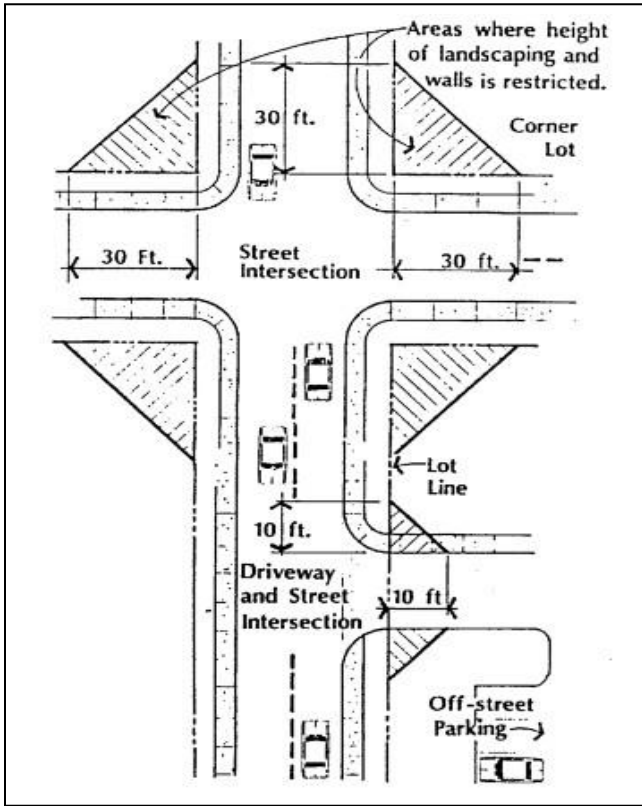
Figure 9-43, Visibility Triangle
