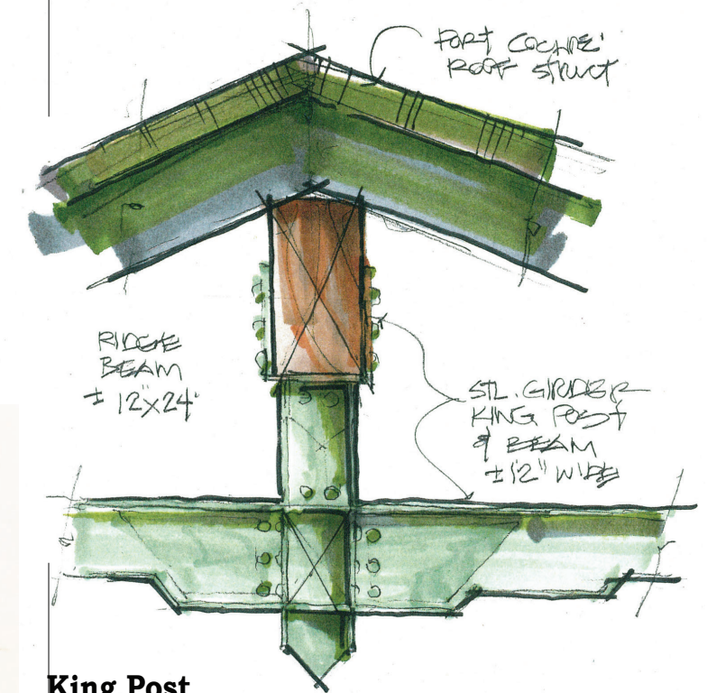
King Post
