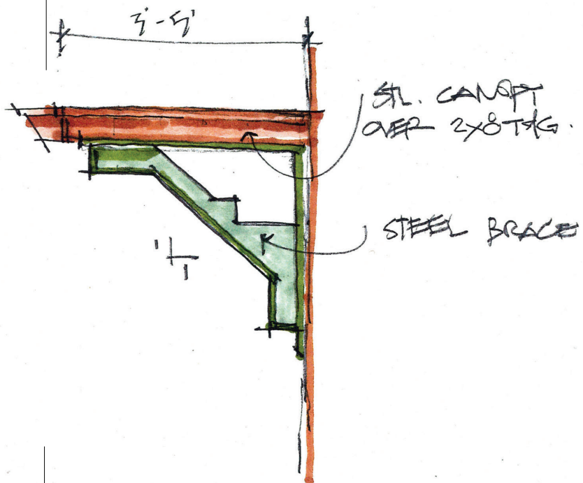
Canopy Brace
