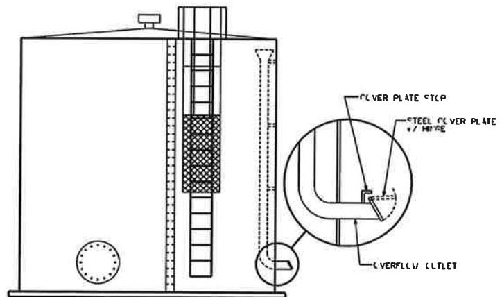
PROFILE VIEW
