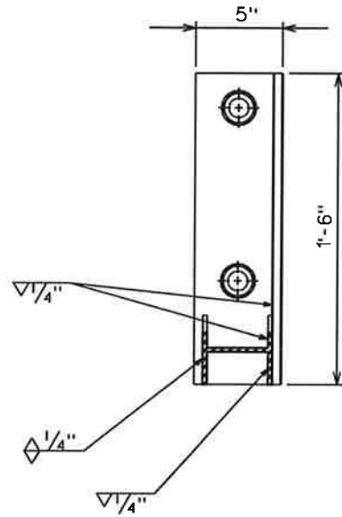
SECTION X-X
