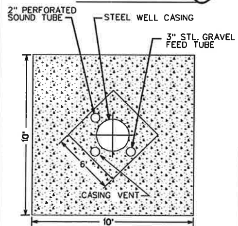
PLAN VIEW CONC. WELL SLAB
