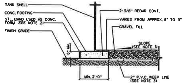
FOUNDATION DETAIL
