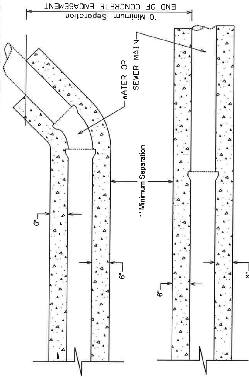
PLAN VIEW
