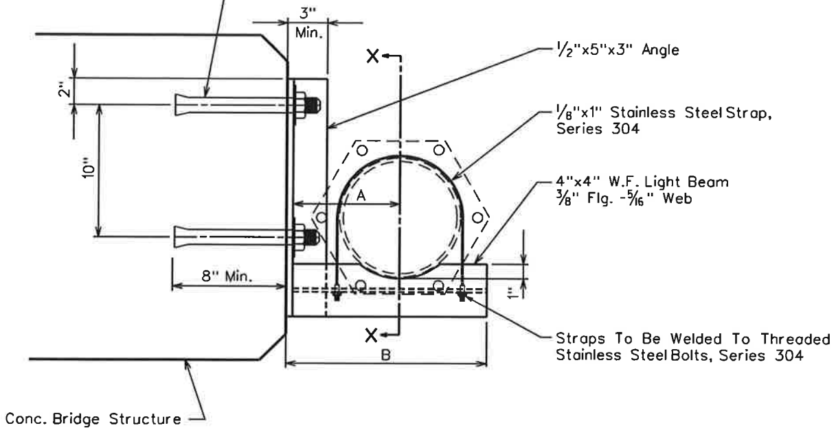
SUSPENSION DETAIL
