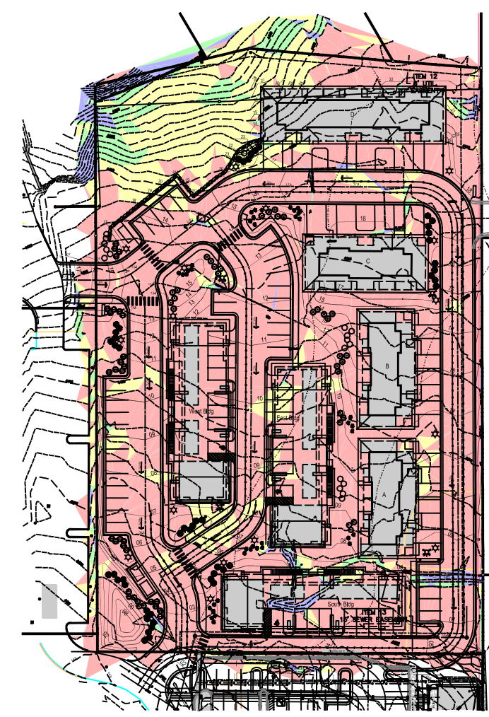
Slope Analysis Scale: 1" - 100'
