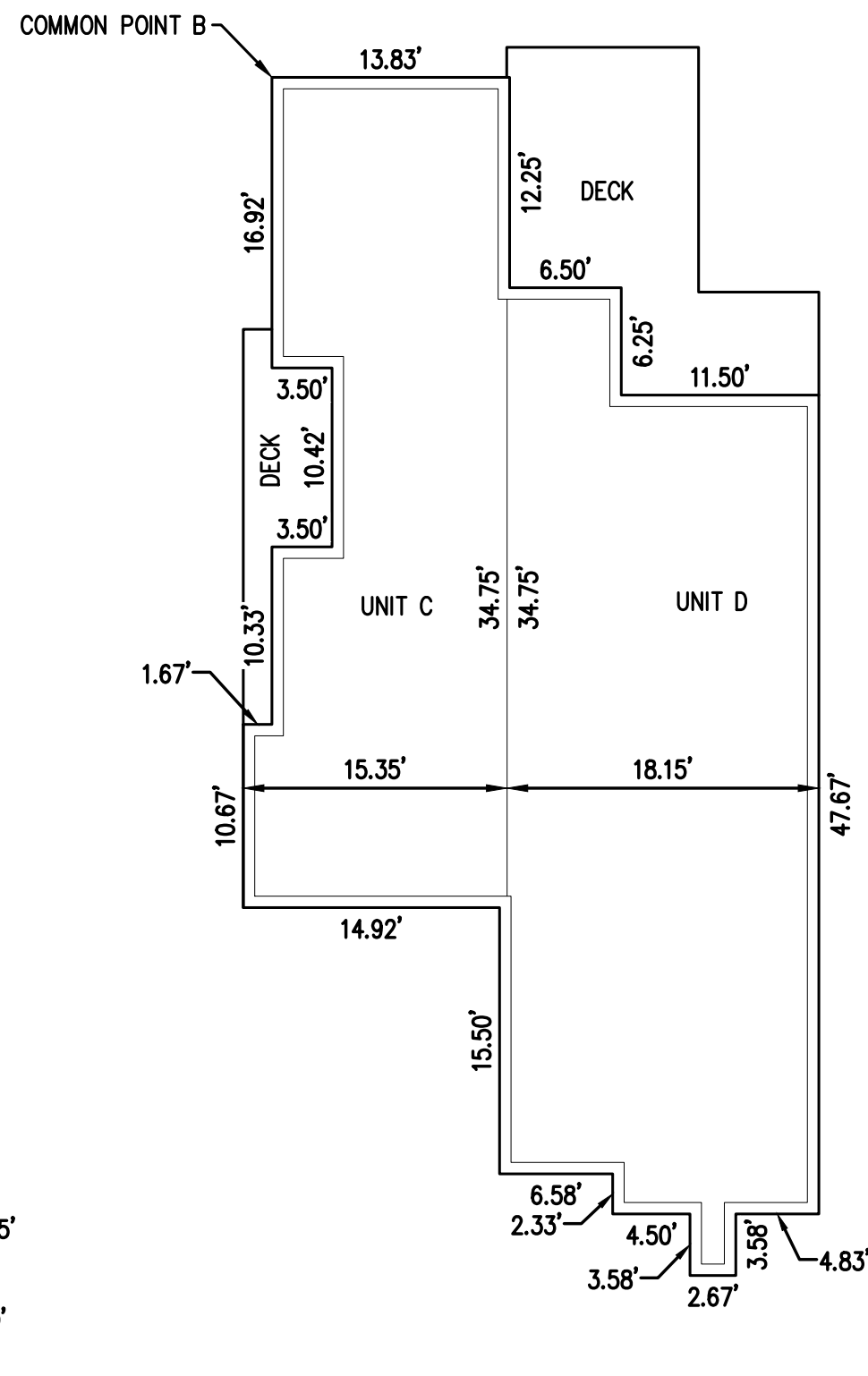
SECOND FLOOR EXTERIOR WALL DIMENSION
