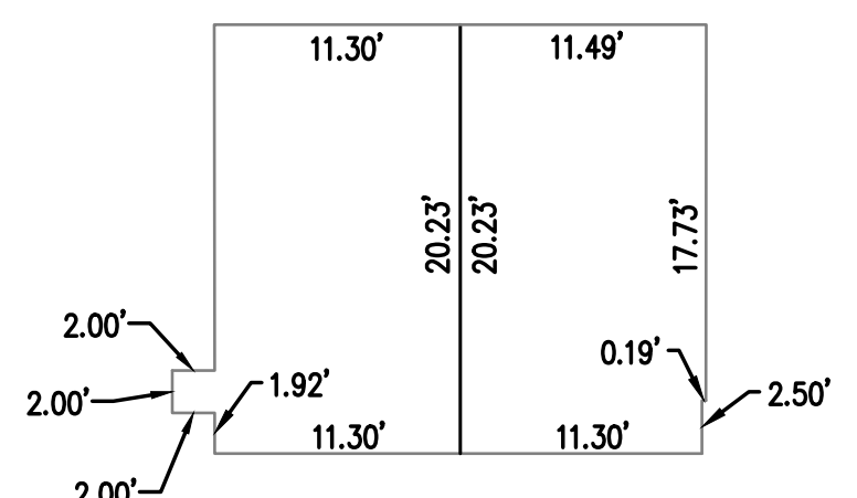
GARAGE INTERIOR WALL DIMENSION
